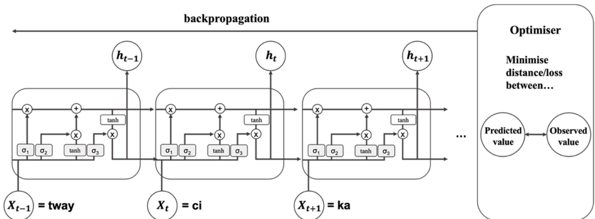
Fig. 2. Model training: LSTM (e.g., twayci-ka ‘pig-NOM’).
