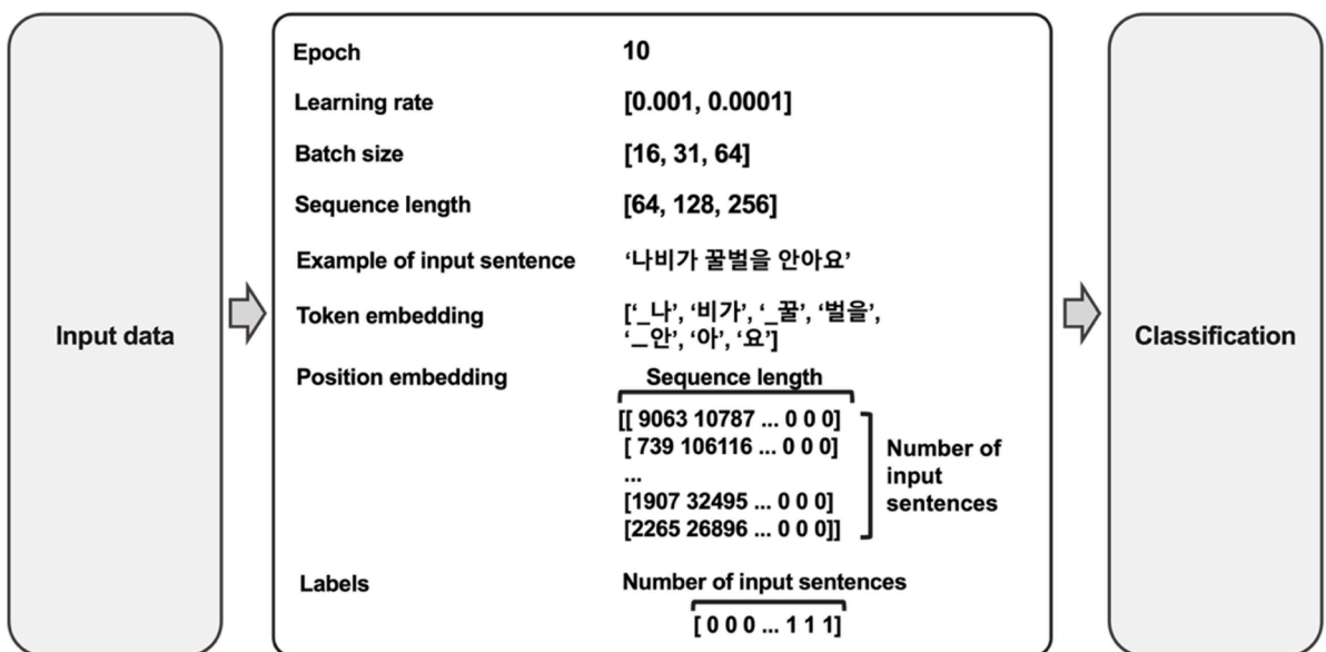
Fig. 3. Model training: GPT-2 (e.g., napi-ka kkwulpel-ul an-ayo butterfly-NOM honeybee-ACC hug-SE ‘The butterfly hugs the honeybee.’).
